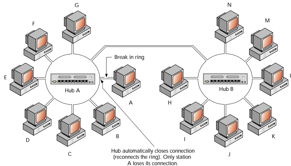
Figure 14 Physical star-wired ring topology
