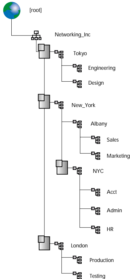
Figure 46 Directory partitions
