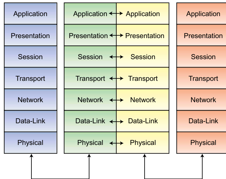
Figure 30 Gateways provide protocol translation between dissimilar systems at more than one OSI layer.
