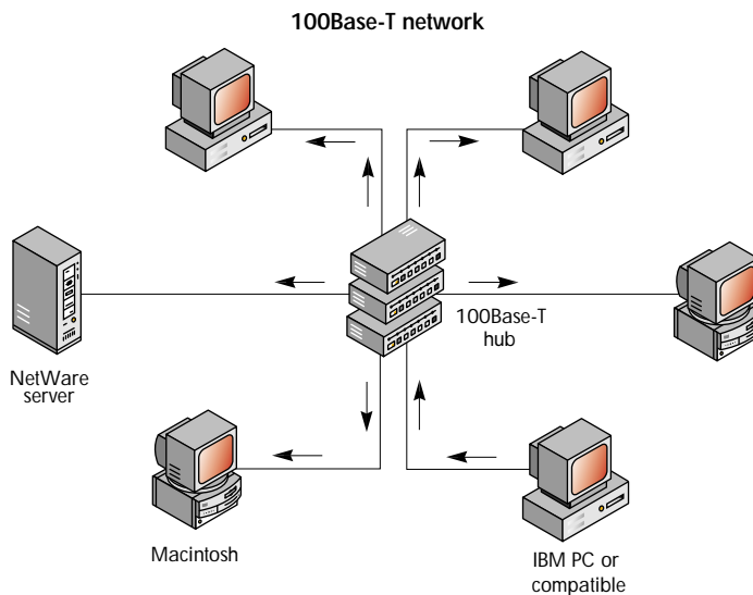
Figure 37 On 100Base-T networks, the physical topology is a star and the logical topology is a bus. A broadcast signal travels to all parts of the cable.
