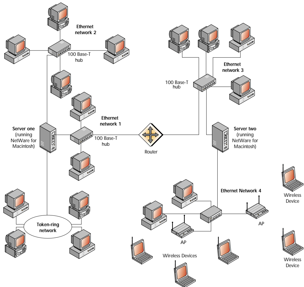
Figure 34 illustrates the two-server internetwork described above.
