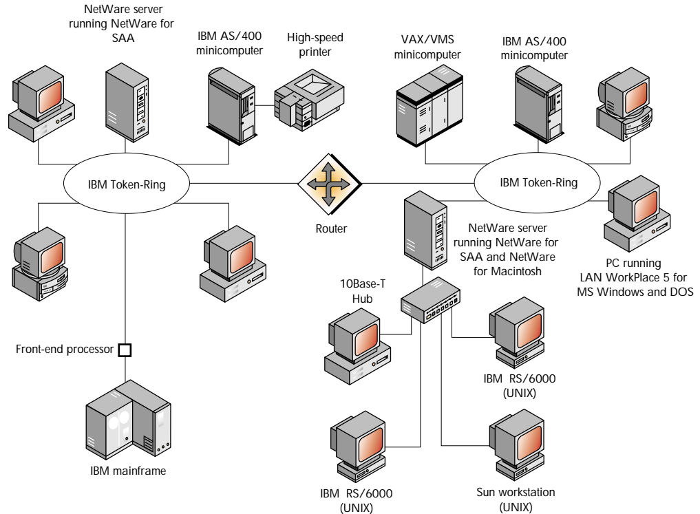
Figure 35 Host systems connected to a complex multiserver NetWare network
