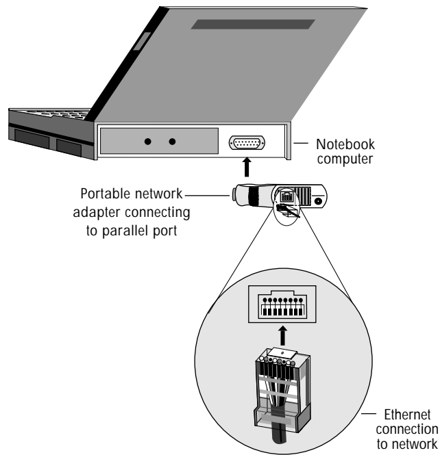
Figure 6 An RJ-45 connector links the adapter to the transmission media.
