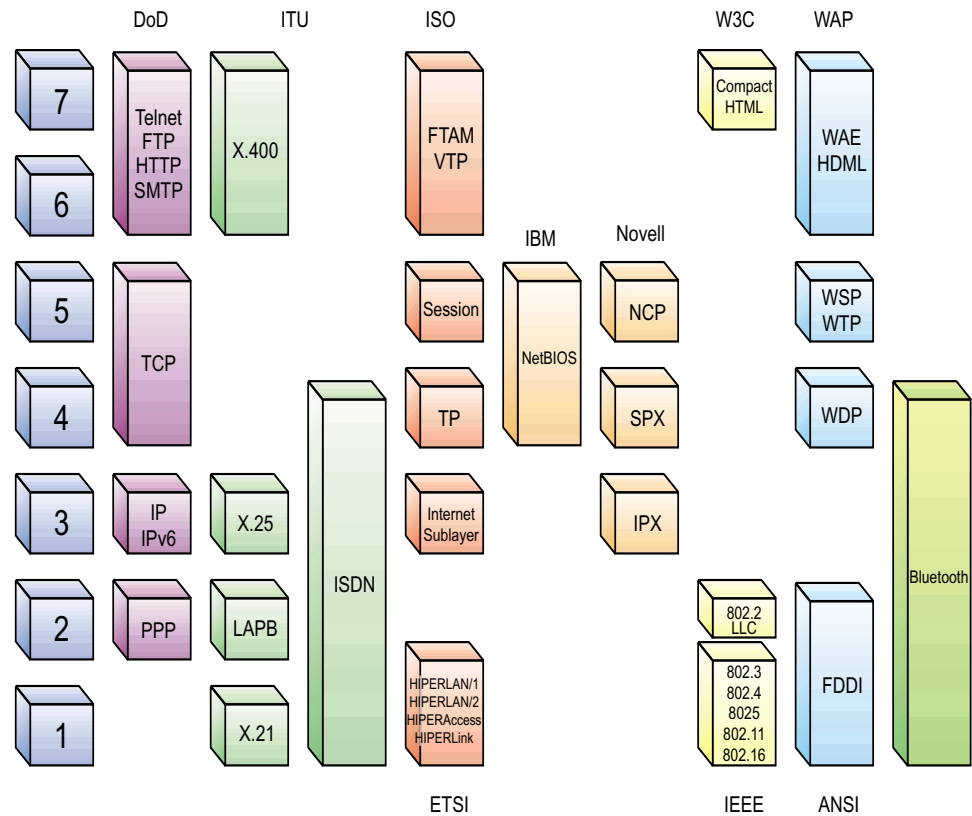
Figure 4 Important standards at various OSI layers
