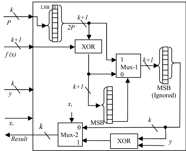
Figure 2. GF(2^k) modulo reduction hardware.
