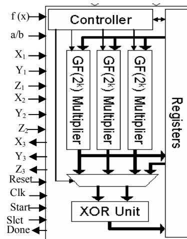
Figure 7. General elliptic curve point hardware outline.
