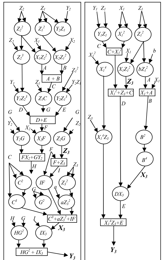
Figure 6. Data flow graphs for the elliptic curve point operations of projecting (x, y) to (X/Z^2, Y/Z^3) .
