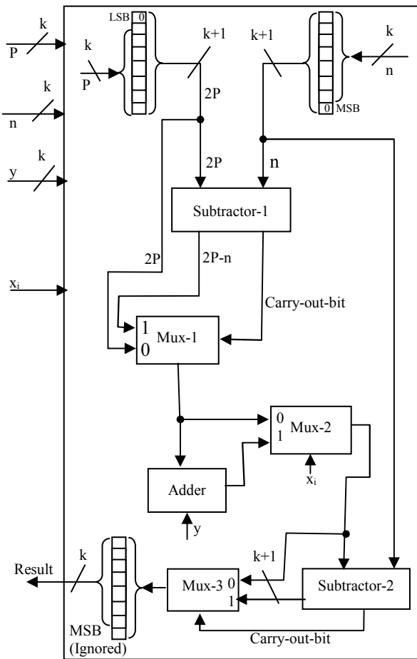
Figure 1. GF(p) modulo reduction hardware.
