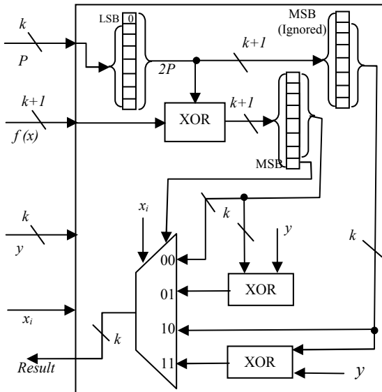
Figure 3. Modified GF(2^k) modulo reduction hardware.
