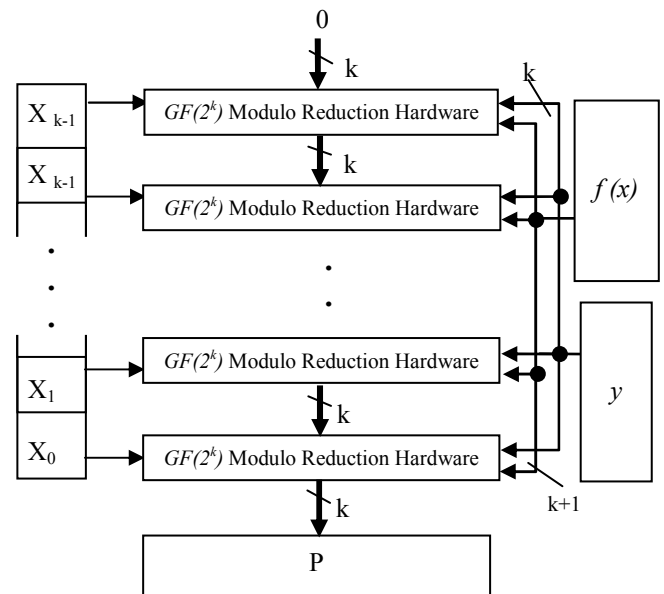
Figure 4. Unfolded GF(2^k) parallel multiplier.
