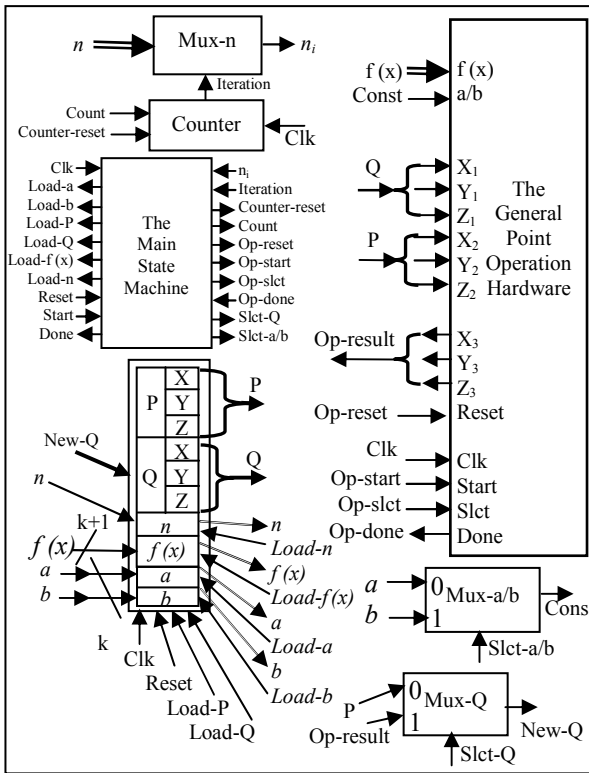
Figure 8. Proposed ECC coprocessor hardware.
